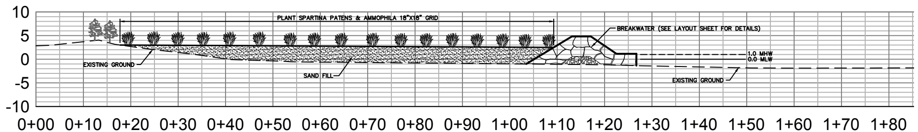
SECTION B-B
