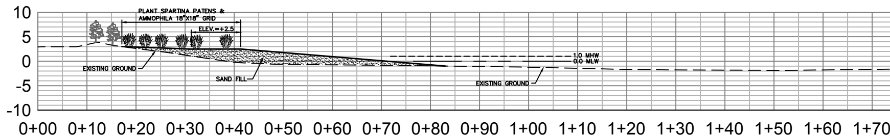
SECTION C-C
